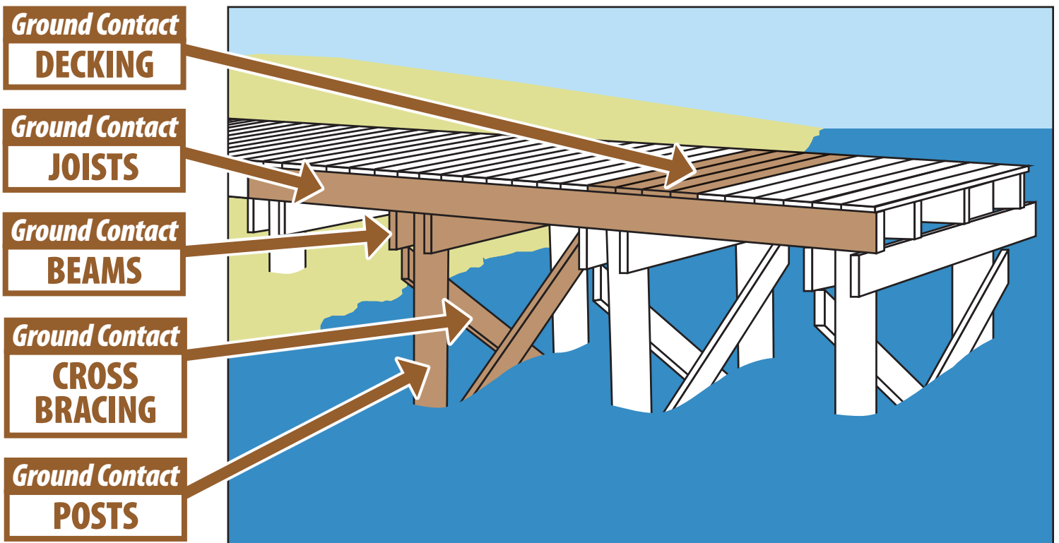
Fresh Water Stationary Dock
