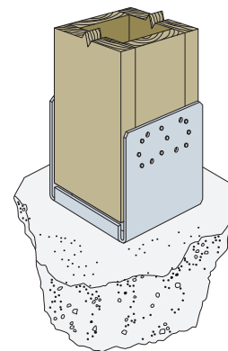
ABU88Z Installed onto 8x8 Culpeper Column
